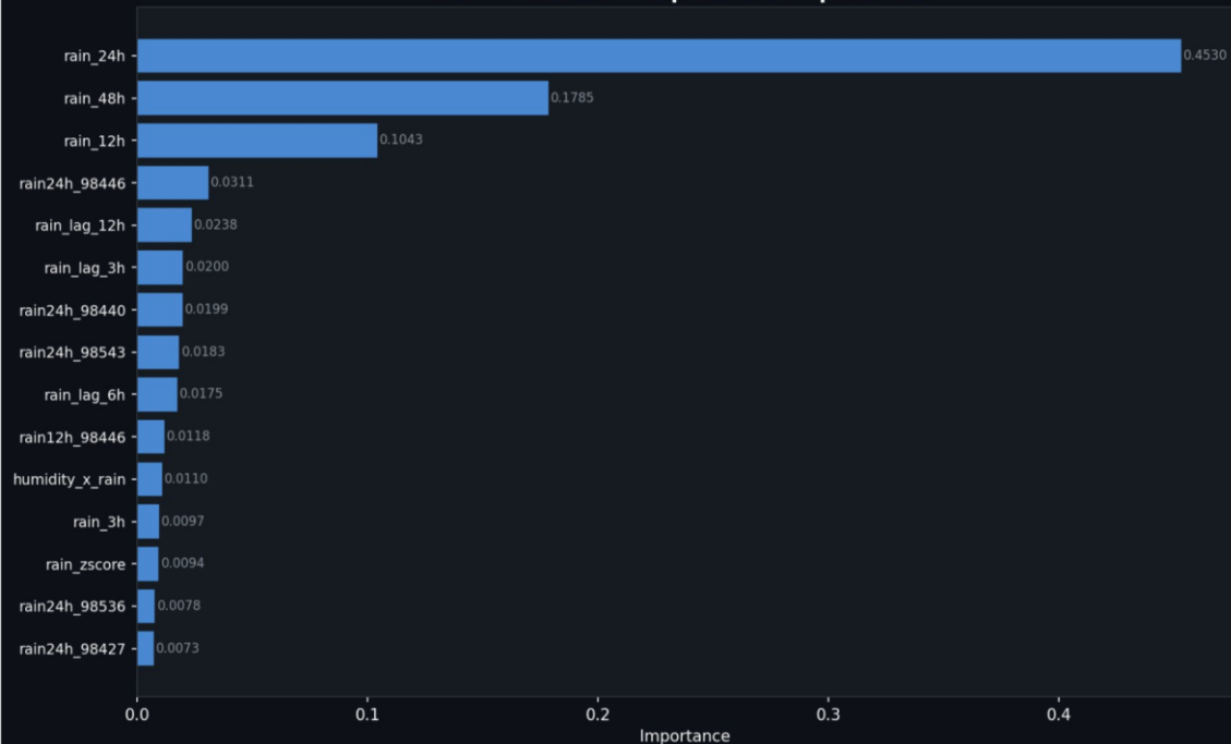
Random Forest — Top Feature Importances
